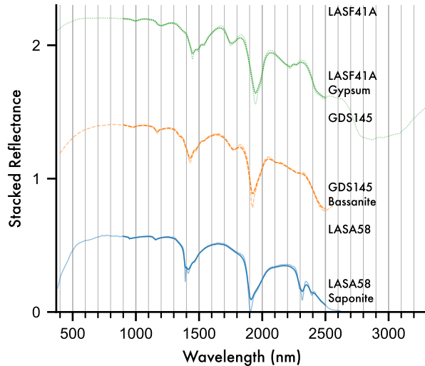
Entfys_Ingaas_Mwir Sampled Gds145 Bassanite, Lasf41A Gypsum, Lasa58 Saponite grouped by Sample Id with Noise
